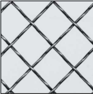
WG100 1/16" ROUND WIRE DOUBLE CRIMPED 3/4" MESH OPENINGS
