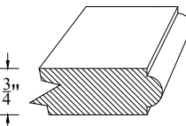
MINI CROWN EDGE: $6.00/LINEAR FOOT AVAILABLE ON 3/4” THICK MATERIAL ONLY.
