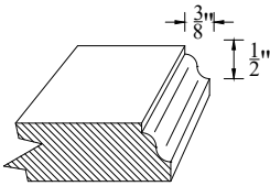
STYLE “B” EDGE: $3.00/LINEAR FOOT (3/8” RADIUS)
