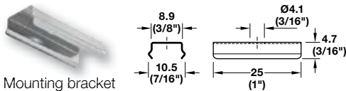
Mounting bracket for concealed fixing
