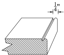
CAMBRIDGE BEAD EDGE: $3.00/LINEAR FOOT
