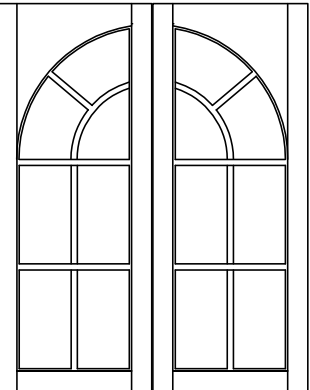
QCL-2000 QCR-2000 QUARTER CIRCLE W/ RADIUS MULLIONS
