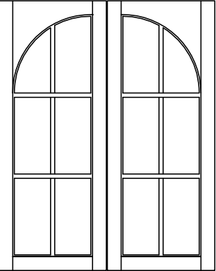
QCL-1000 QCR-1000 QUARTER CIRCLE W/ STRAIGHT MULLIONS
