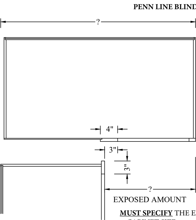
FRAMELESS BLIND BASE DETAIL
