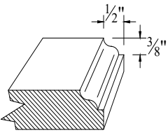
CORNER BEAD EDGE: $3.00/LINEAR FOOT
